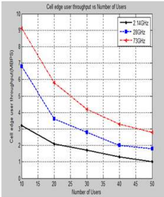
Fig: 6 28 and 73GHz at 10mbps
